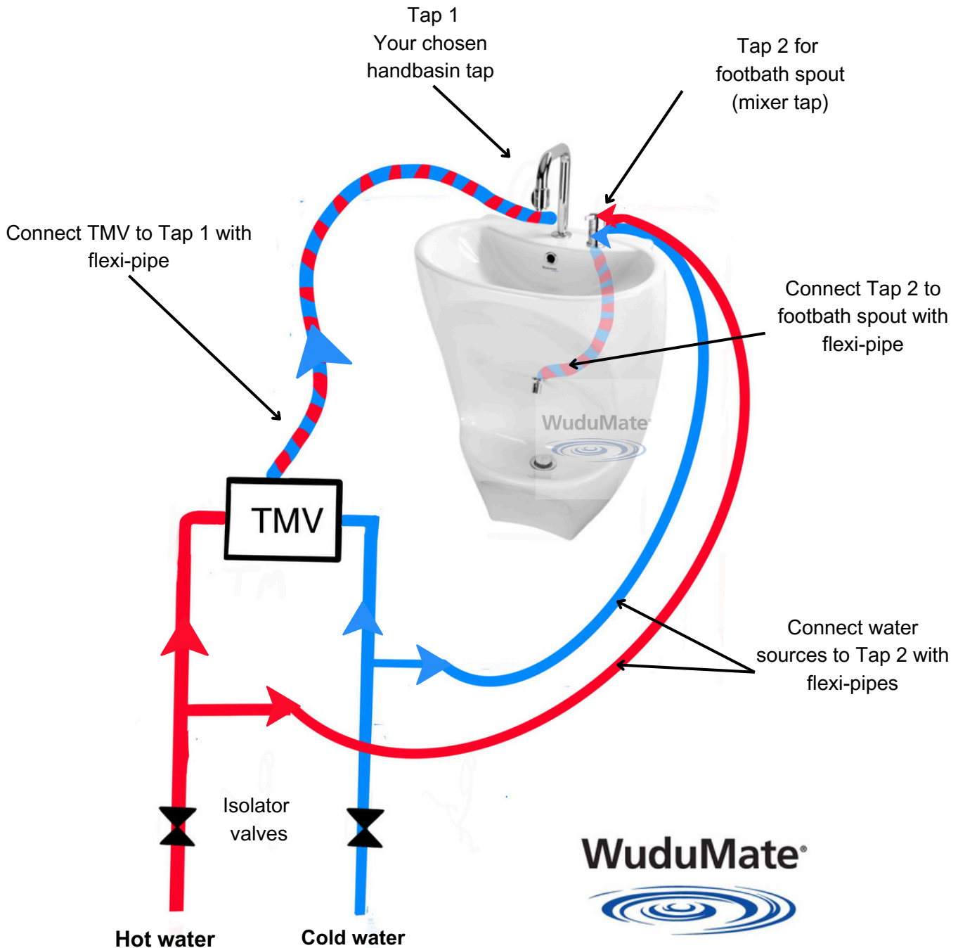
Diagram1.1: Pre-mixed water to basin, footbath manually controlled
